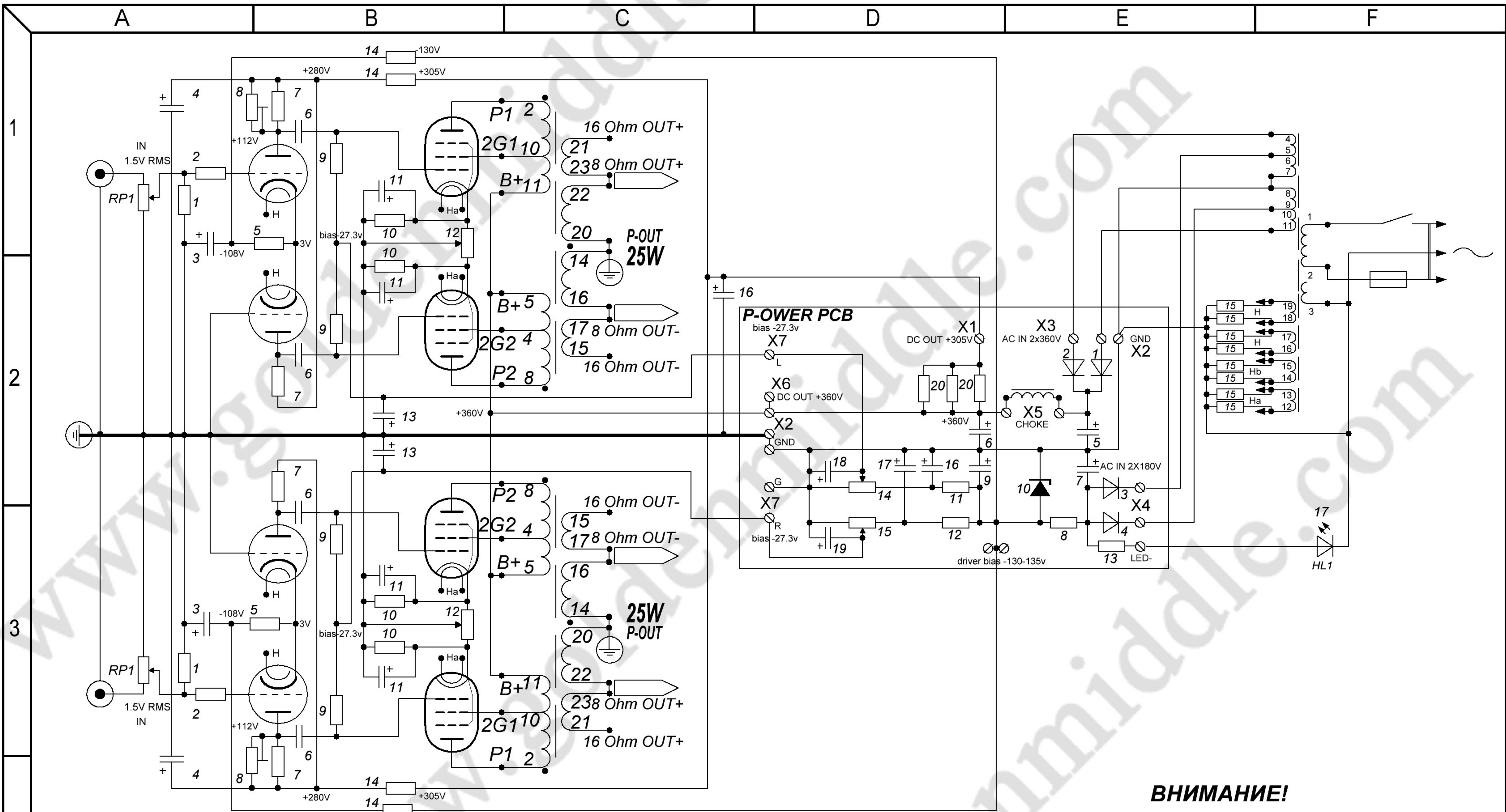
6П3С/6L6GC
