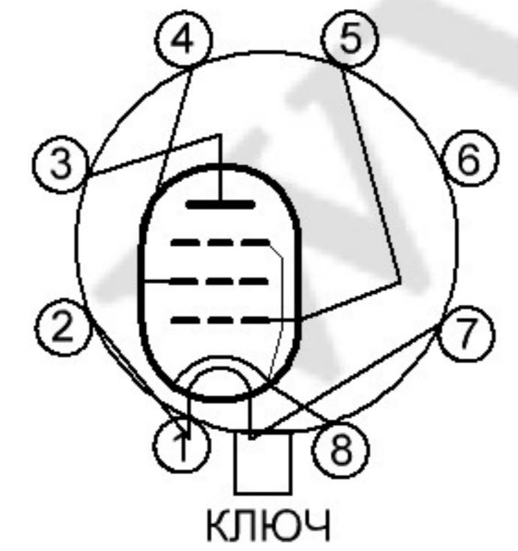
6П3С/6L6GC
